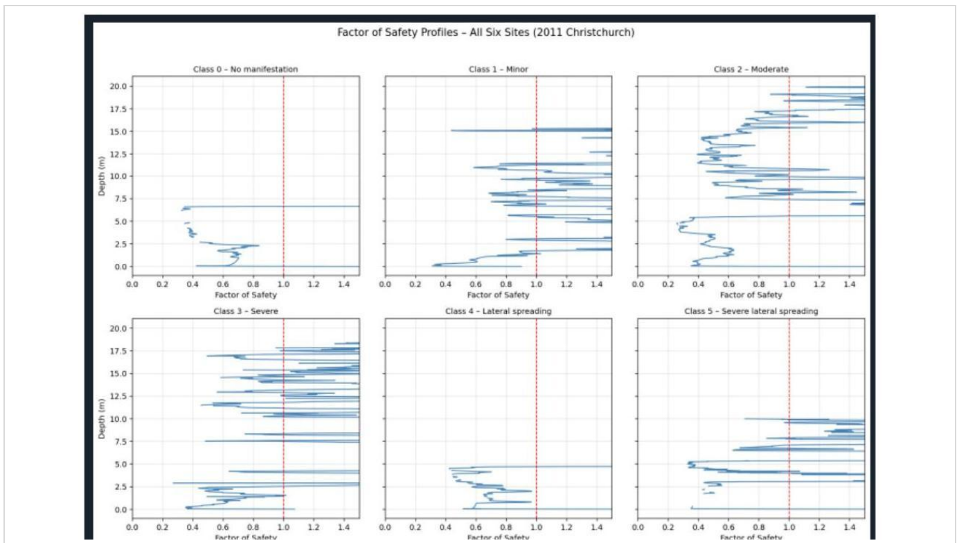
Figure 3. Factor of safety profiles versus depth for all six selected CPT sites (measured data).
