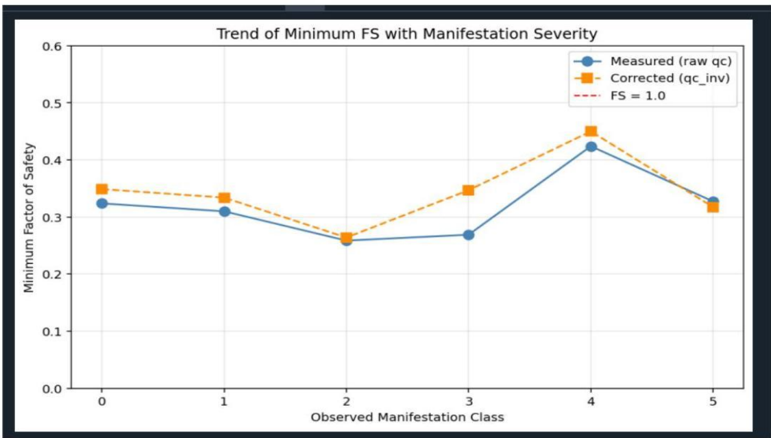
Figure 2 Trend of minimum FS across observed manifestation classes (measured vs. thin-layer-corrected). No consistent downward trend, FS dips at Class 2, peaks at Class 4, and Class 0 sits almost on top of Class 5.
