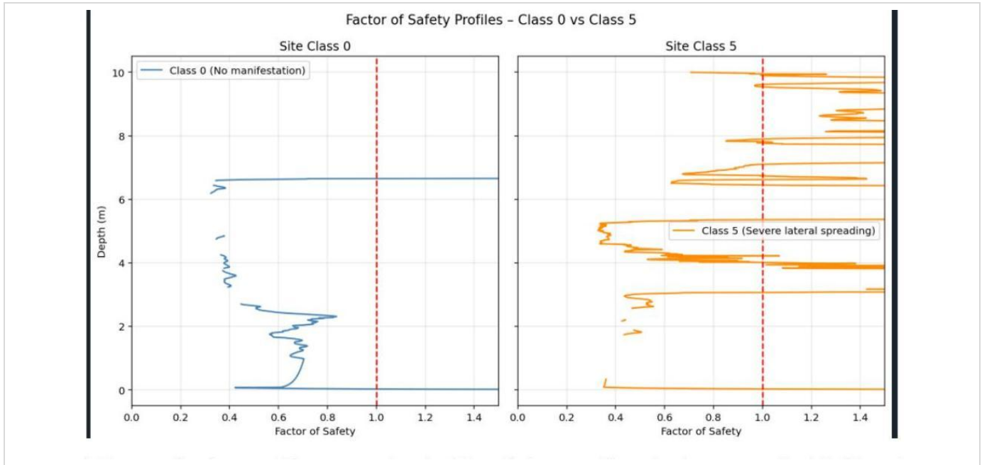
Figure 4. Factor of safety profiles versus depth: Class 0 (no manifestation) compared with Class 5 (severe lateral spreading).
